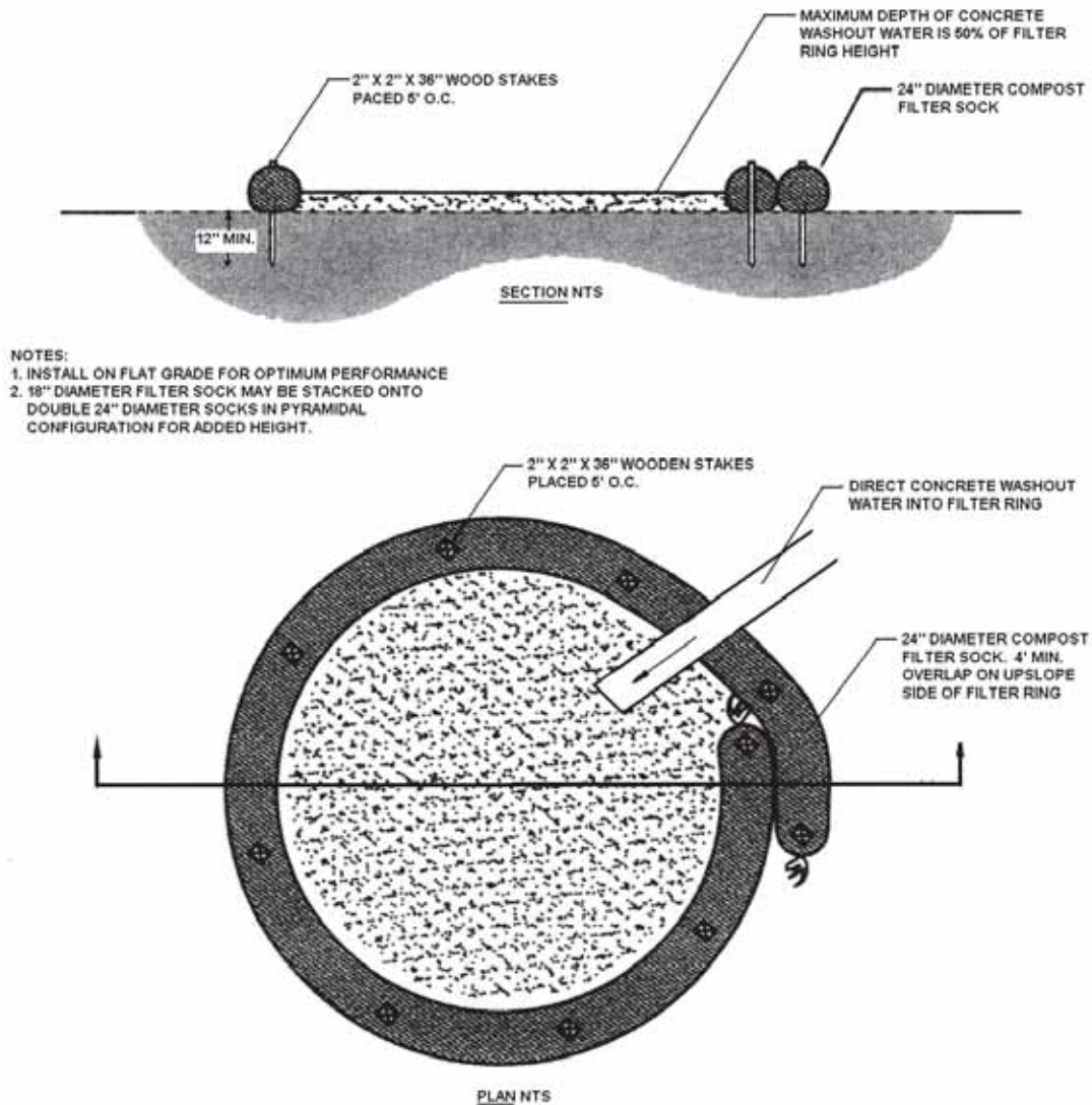
FIGURE 3.18 Typical Compost Sock Washout Installation
