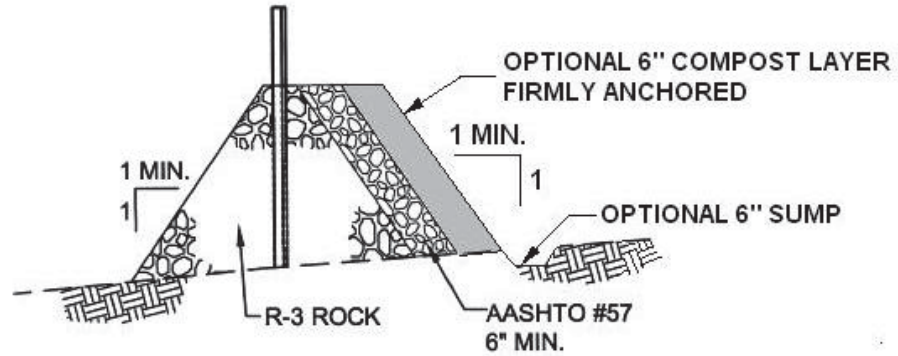
OUTLET CROSS-SECTION
