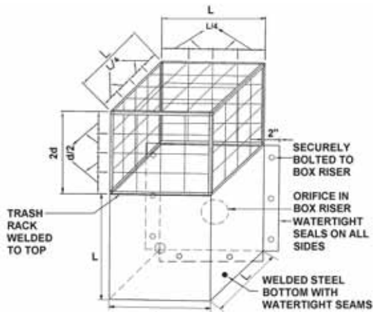
FABRICATED STEEL RISER DETAIL NO SCALE
