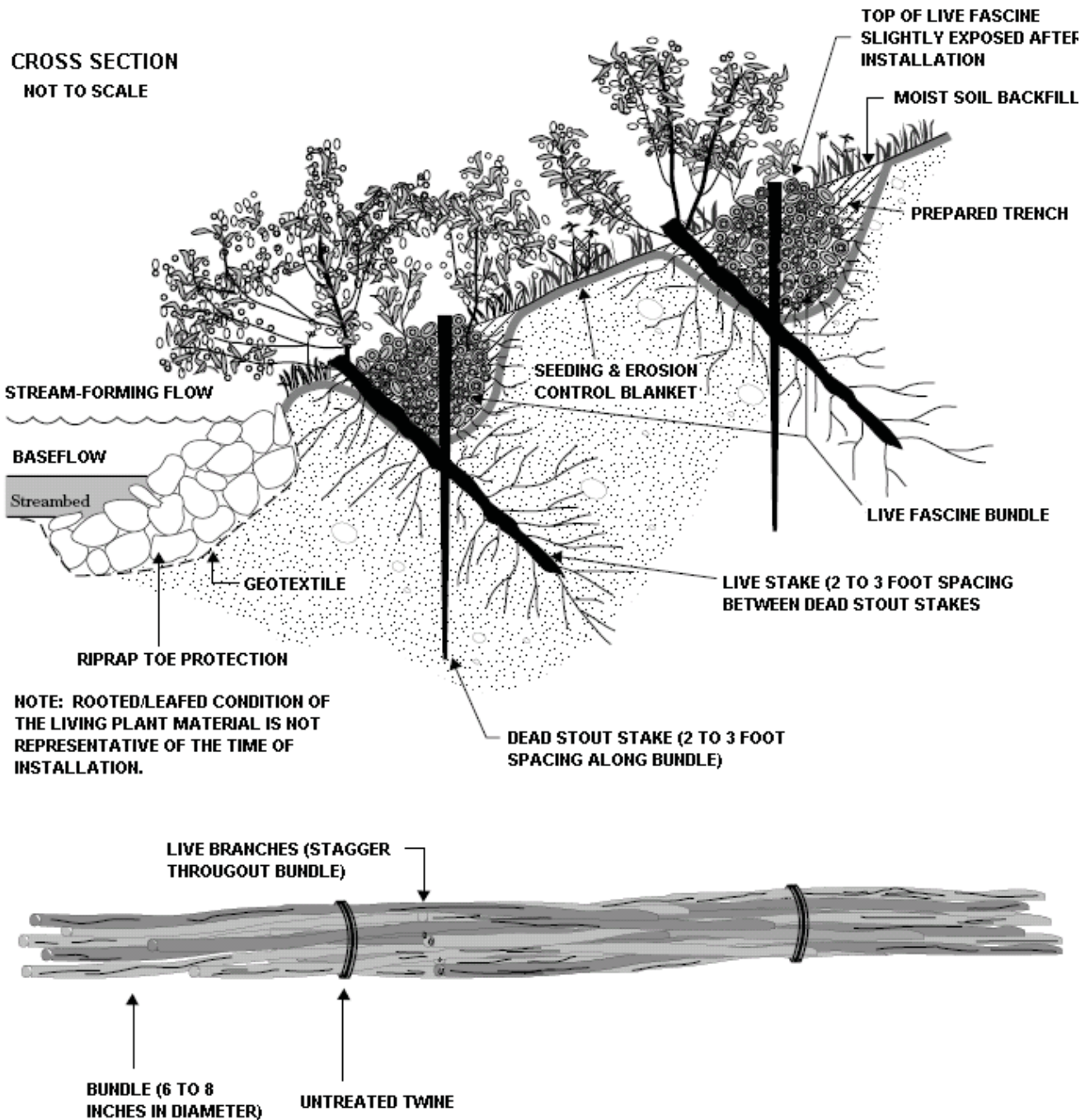
FIGURE 15.7 Live Fascines
