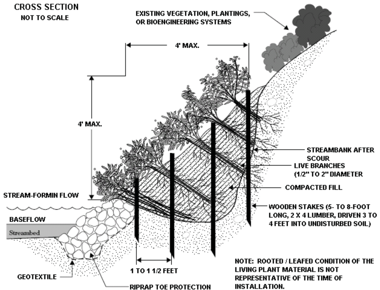
FIGURE 15.8 Branchpacking
