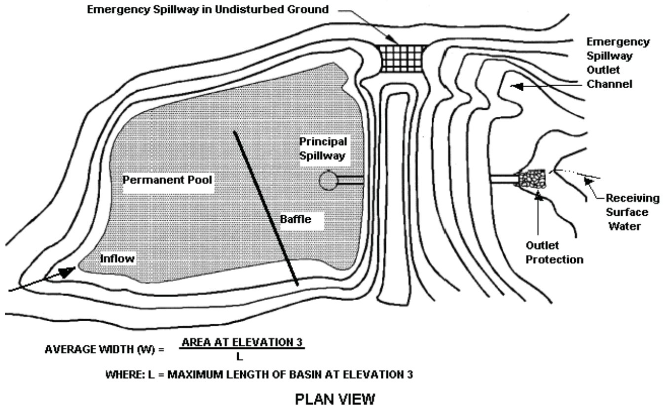
FIGURE 7.1 Sediment Basin
