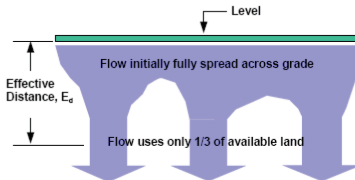
Figure G.7. Concentration of Flow Down Slope of Level Spreader
