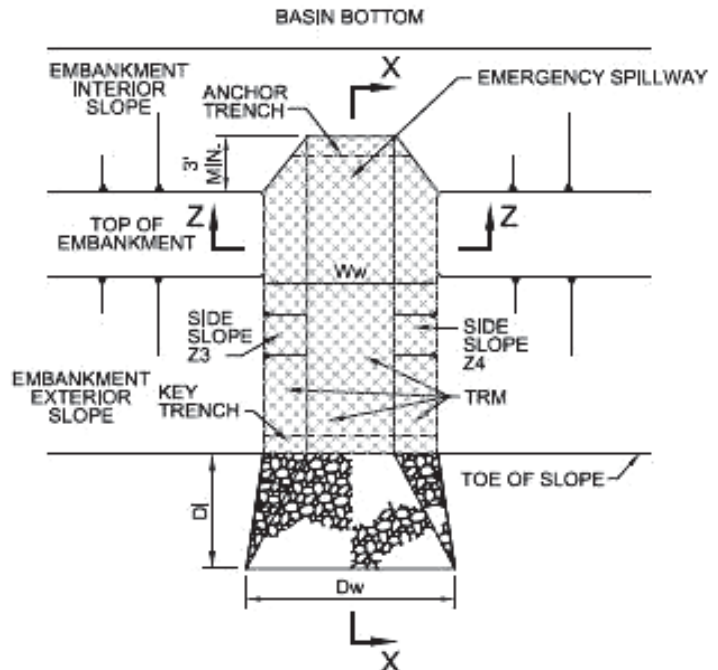
PLAN VIEW RIPRAP OUTLET DISSIPATOR
