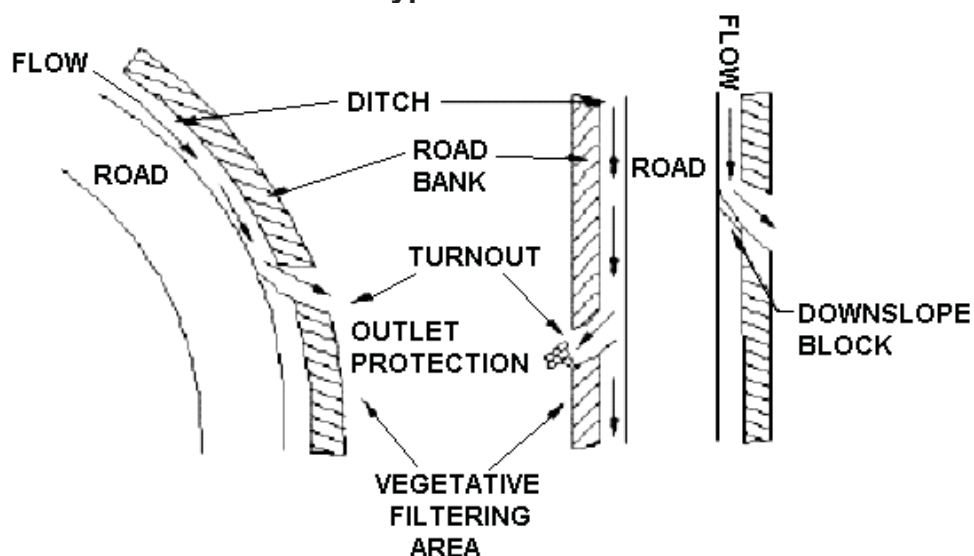
FIGURE 3.3 Typical Turnout
