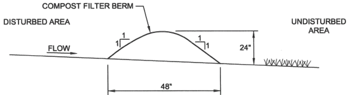
SECTION VIEW
