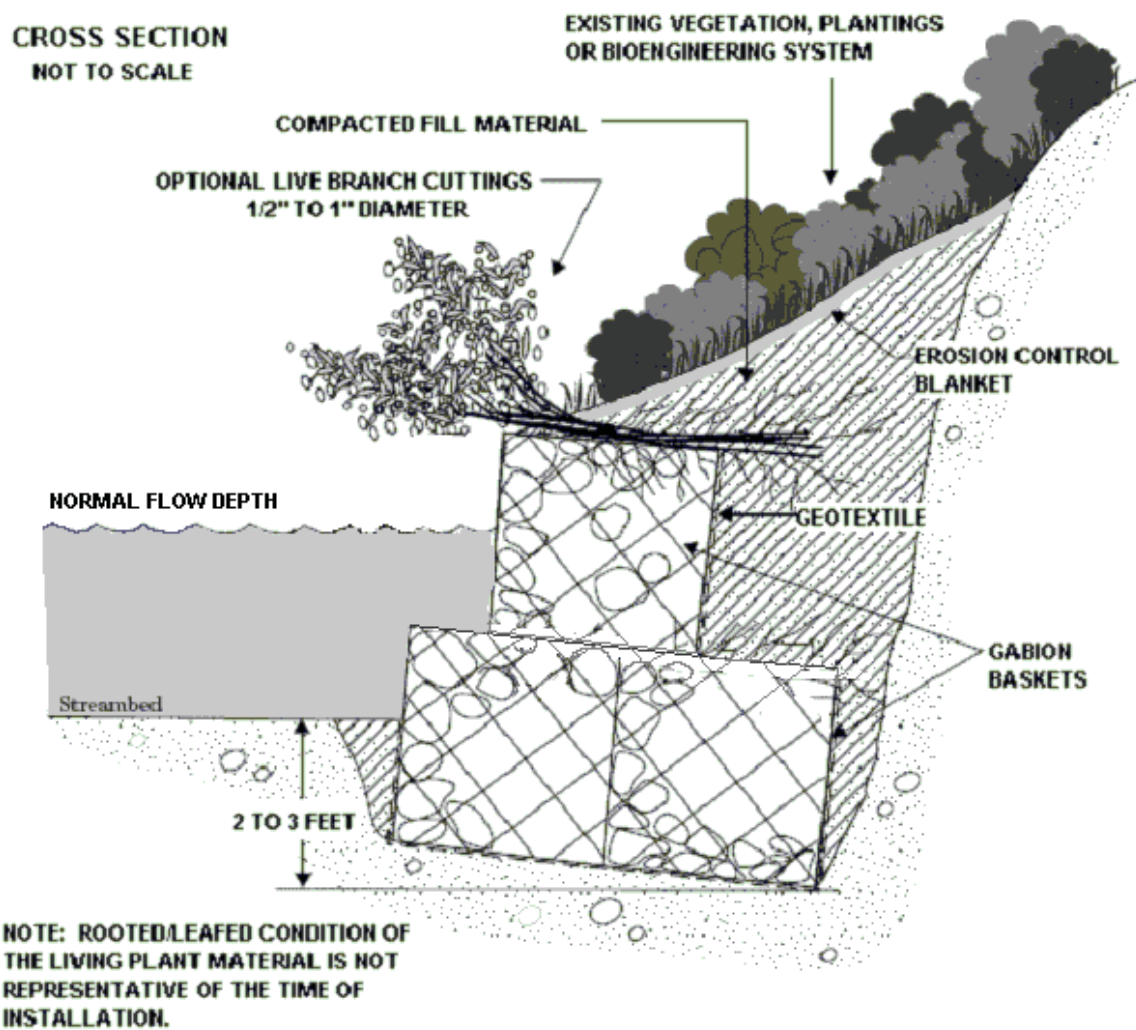
FIGURE 15.3 Gabion Streambank Protection
