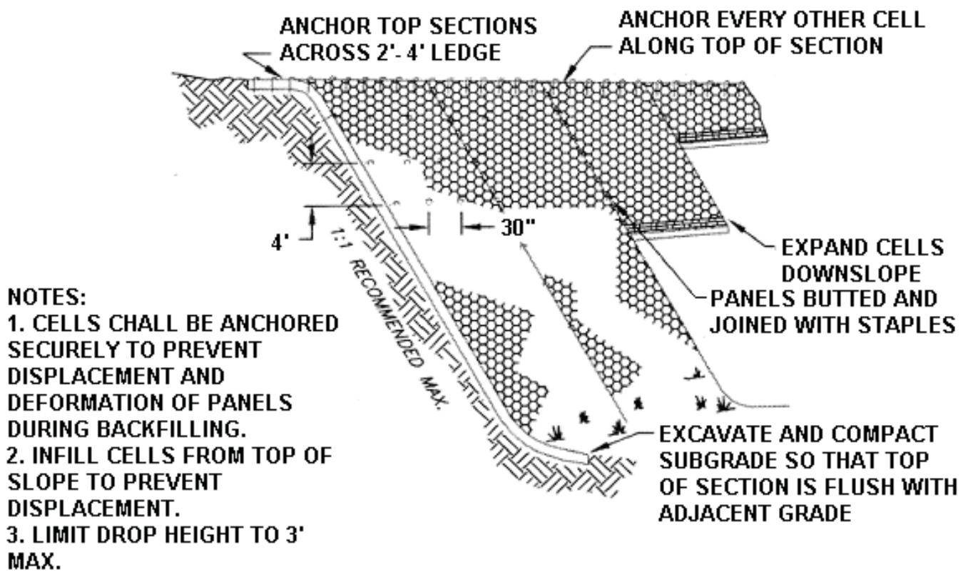
FIGURE 11.6 Typical Cellular Confinement System Installation
