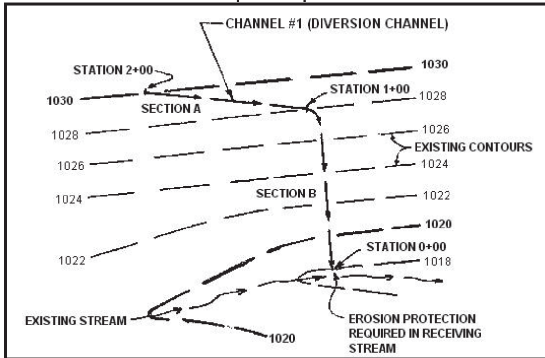
FIGURE 6.3 Plan Map of Sample Channel
