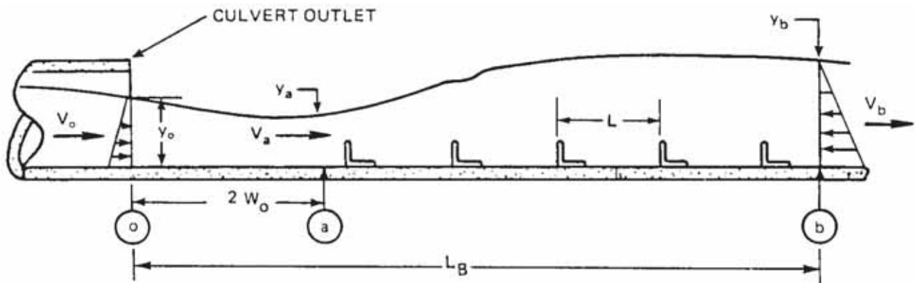
FIGURE F.3 Critical Dimensions Used in Designing Roughness Element Dissipaters
