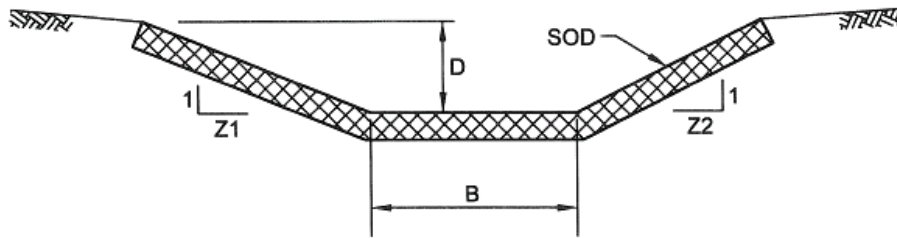
CHANNEL CROSS-SECTION
