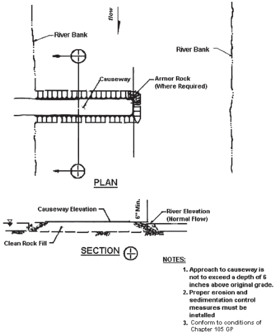
FIGURE 3.8 TYPICAL CAUSEWAY
