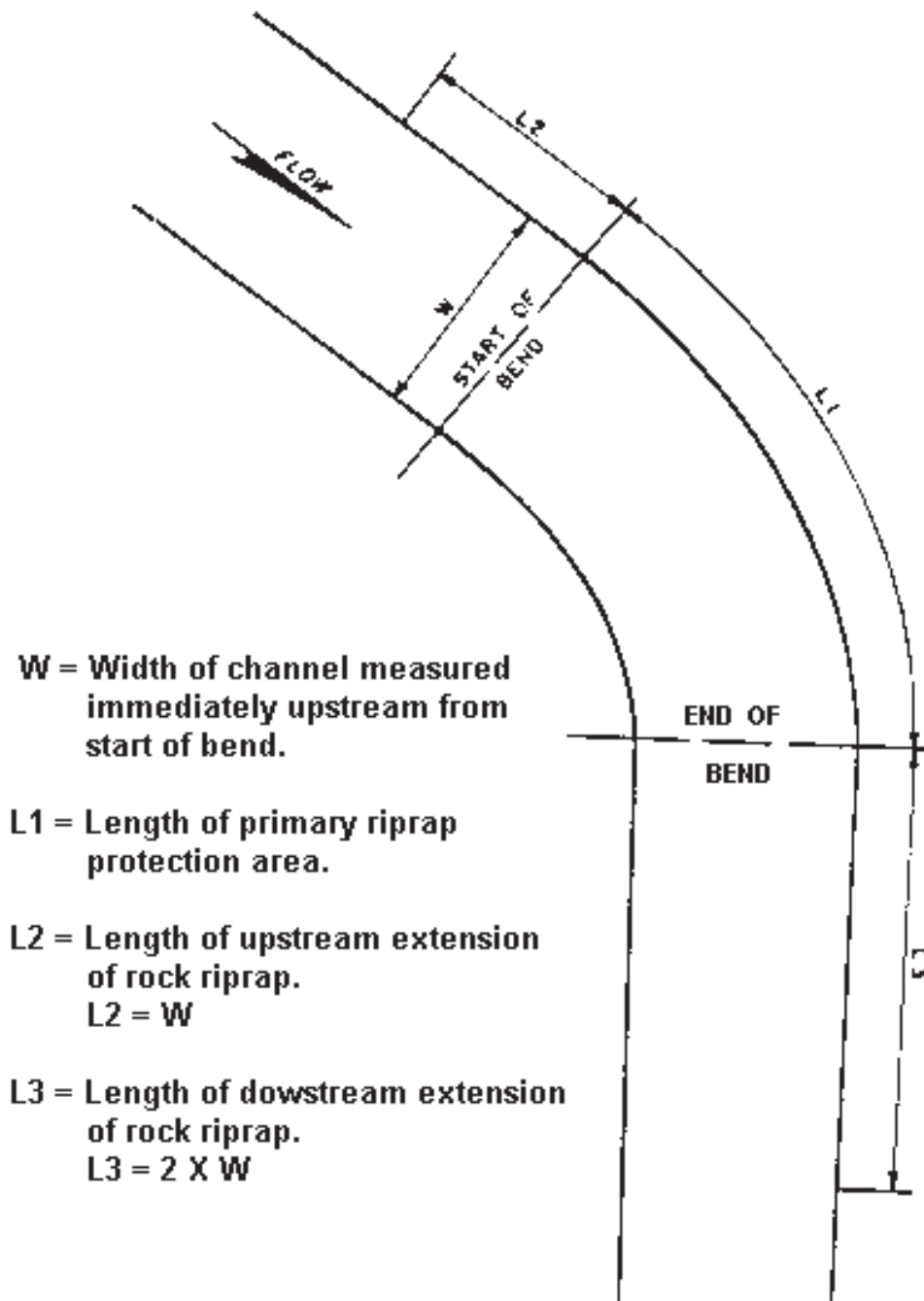
FIGURE 15.2 Extension of Primary Rock Riprap Protection Area
