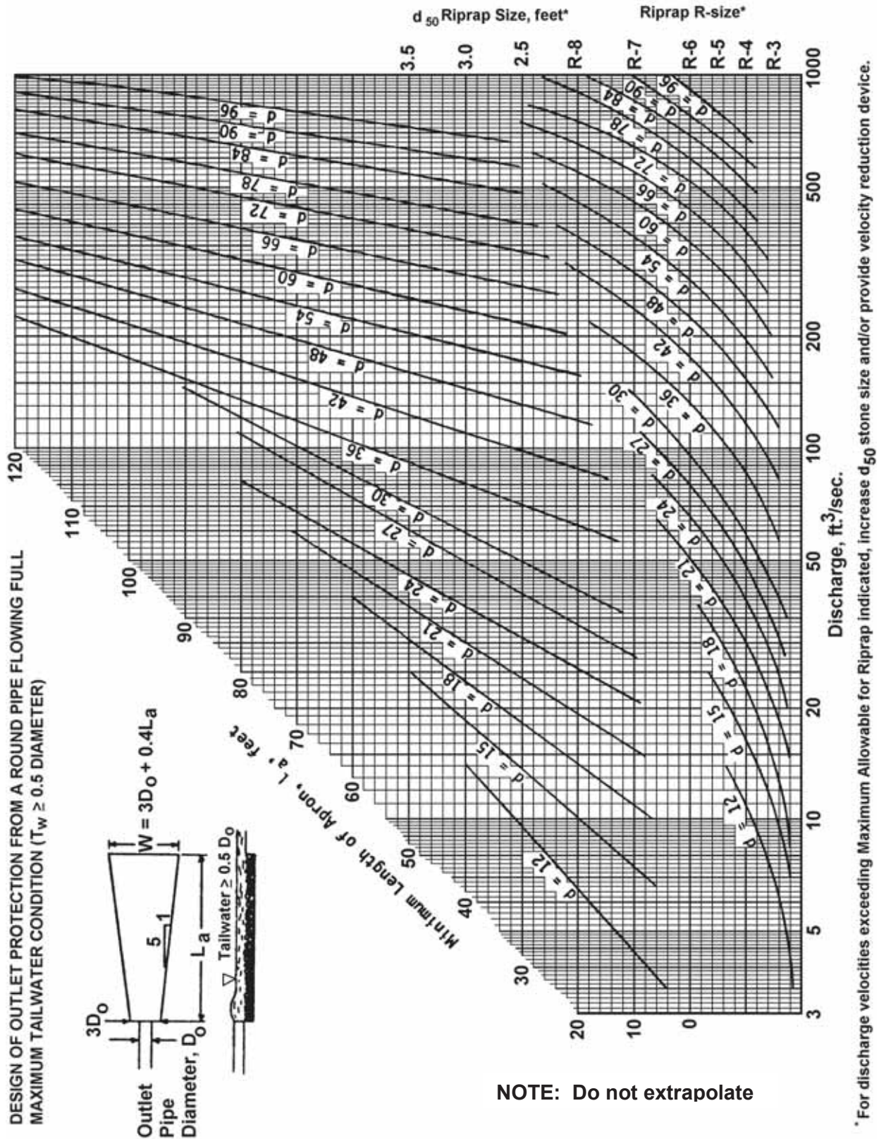
FIGURE 9.4 Riprap Apron Design, Maximum Tailwater Condition
